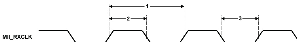
Figure 6-46. MII_RXCLK Timing (EMAC - Receive)
